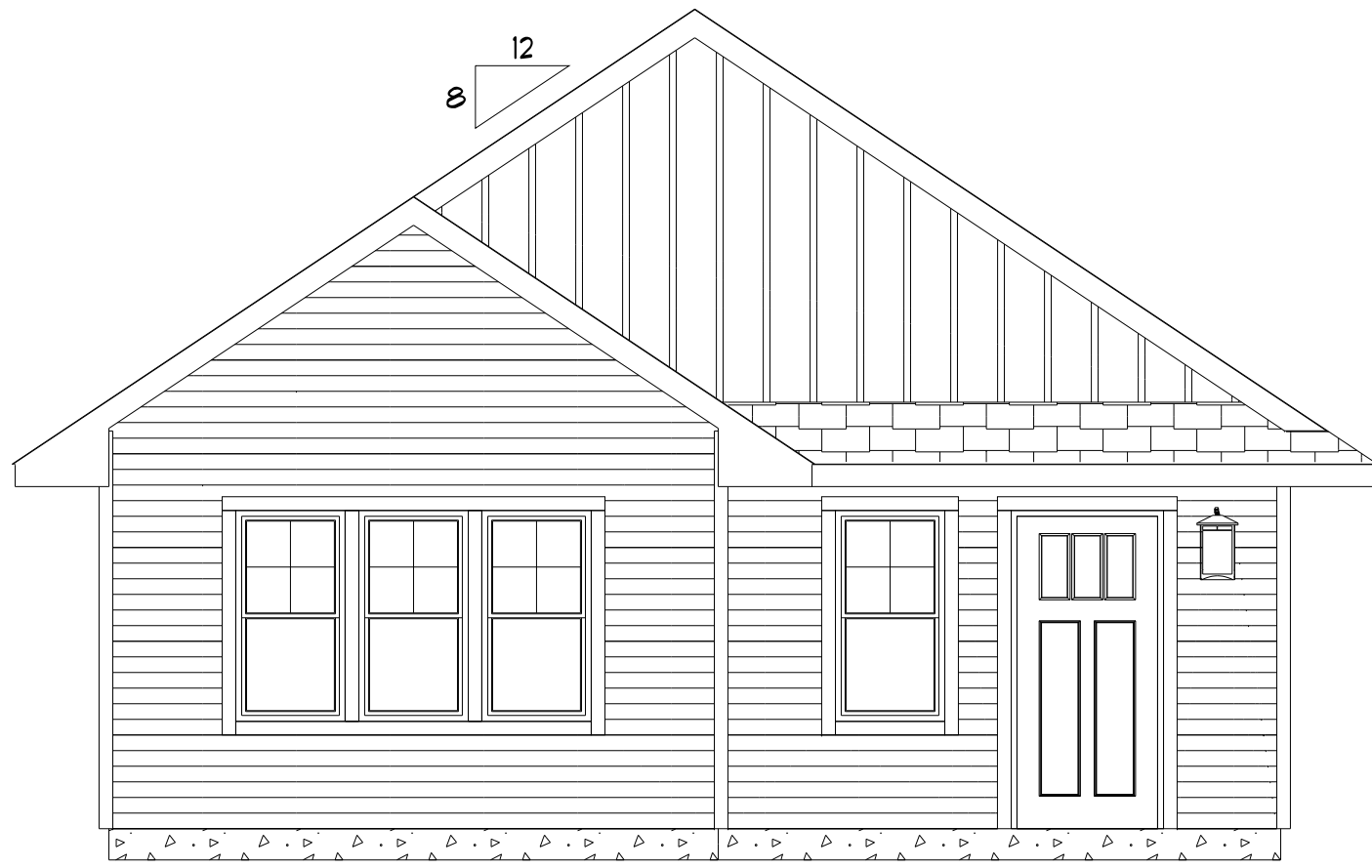
FRONT ELEVATION
