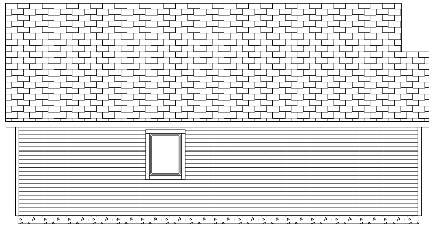
LEFT ELEVATION
