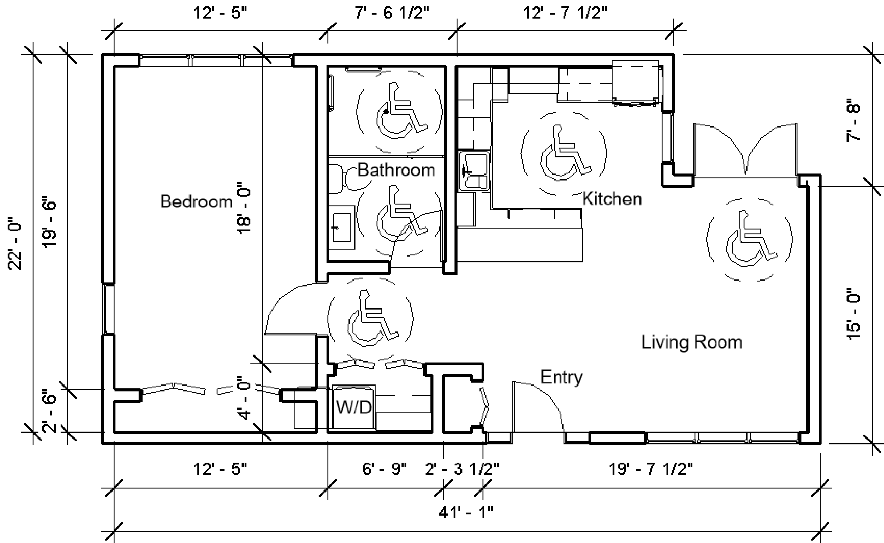
DIMENSIONED FLOOR PLAN | THE INICIO
